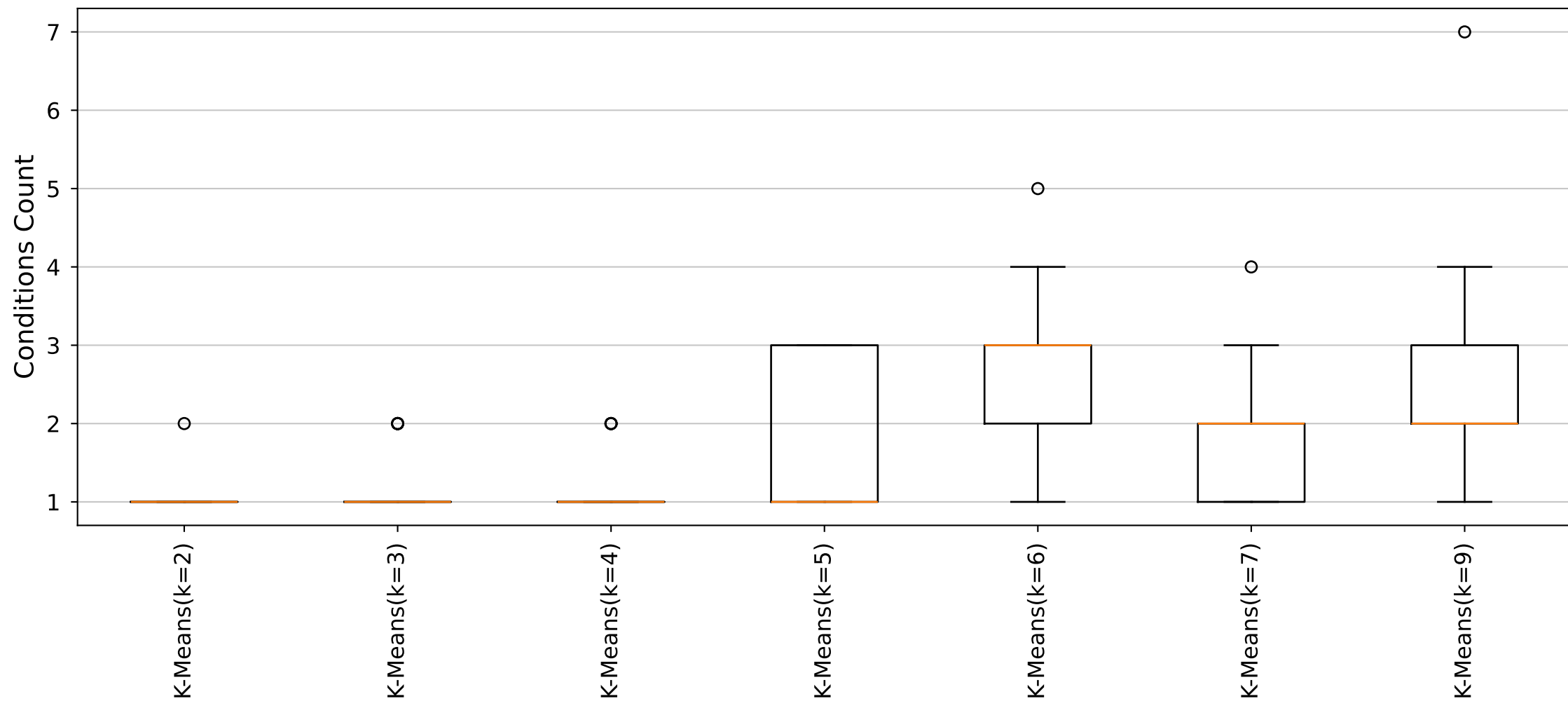
YARA Rules Conditions Count Distribution (Cluster13_Size9 dataset)
